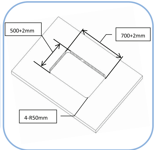
Diagram 1. Cut hole size on roof
