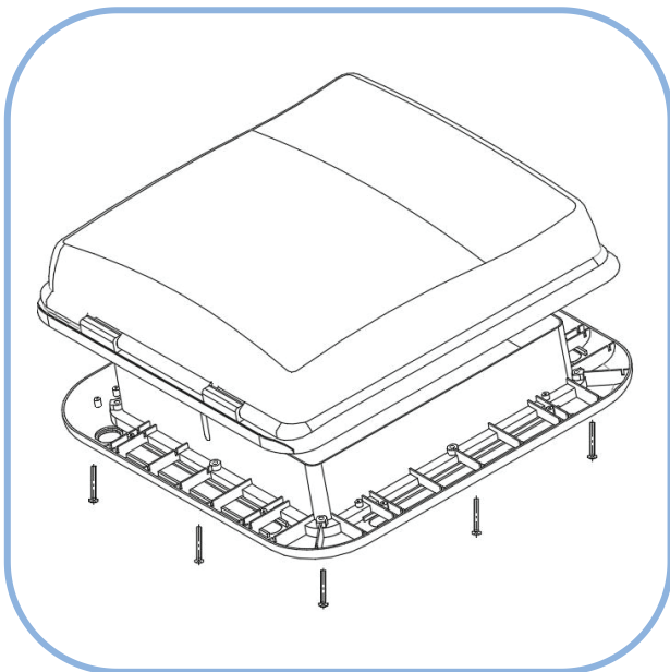
Diagram 5. Screw in the outer shell
