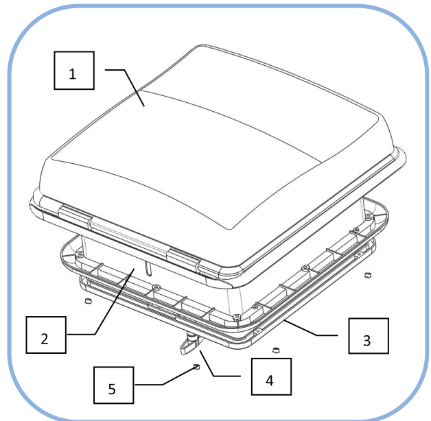
1. Outer shell, 2. Inner shell, 3. Screen frame, 4. Handle, 5. Screw cap (280×280)
