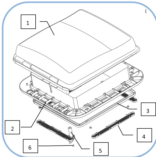
1. Outer shell, 2. Inner shell, 3. Screen frame, 4. Lamp cover, 5. Handle, 6. Screw cap (320×320)
