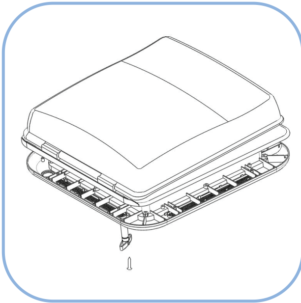
Diagram 7. Install the handle
