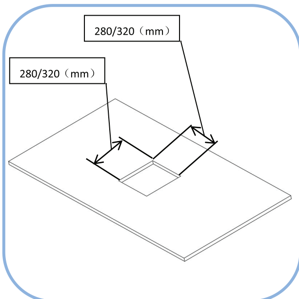
Diagram 1. Cut hole size on roof Size: 320×320, 280×280
